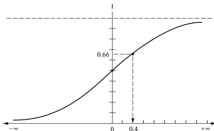
FIGURE 15.5 Normal CDF.
